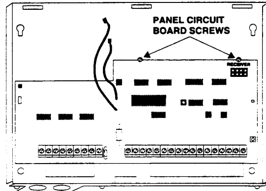
Figure 1. Panel Circuit Board Screw Locations
