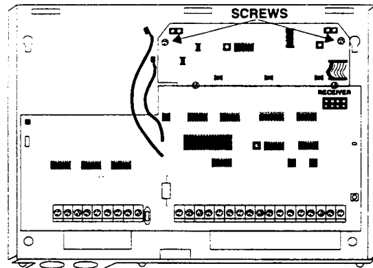
Figure 2. Receiver and Screw Locations
