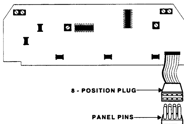
Figure 4. Connecting the 8-Position Plug
