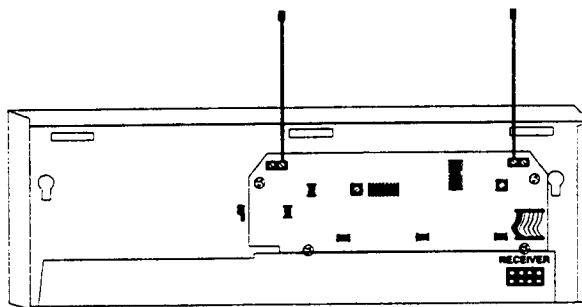
Figure 3. Installing the Antennas
